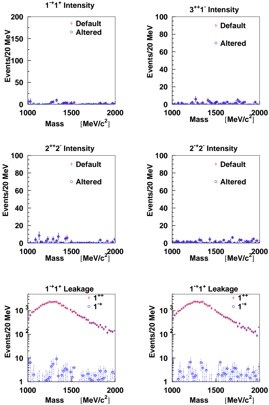
Figure 2: PWA results for reaction 1 using the default geometry specifications. These results show the intensity for the waves that are not physically present in the data set. The 1^{-+} wave is the exotic \pi_1 channel. The bottom two figures show the strength of the leakage into the exotic 1^{-+} wave compared to the strength of the 1^{-++} signal — the latter is believed to be the source of the leakage. The level of the leakage is below 1% for the nominal detector configuration.
